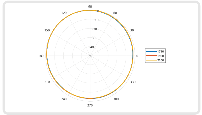
Azimuth: 1710 - 2700 MHz
