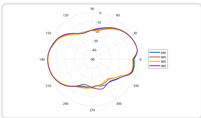
Elevation: 690 - 960 MHz
