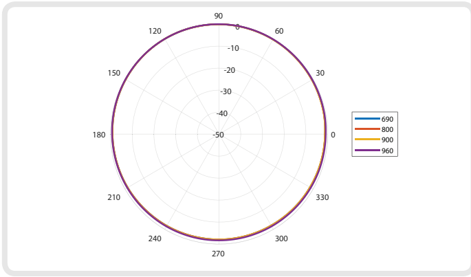
Azimuth: 690 - 960 MHz
