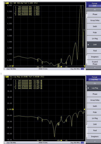
VSWR and Return Loss Model: ANT-868-14dbi-Yagi 14 Elements
