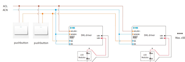
Wiring diagram
