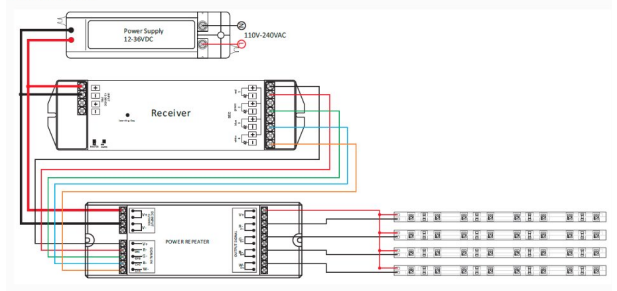
Wiring Diagram
