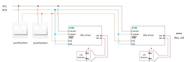
Wiring diagram
