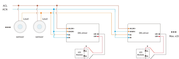
Wiring diagram
