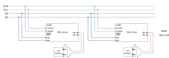
Wiring diagram
