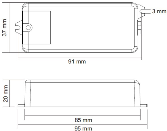
Product Dimension
