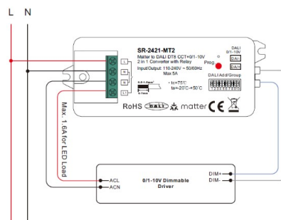
Wiring Diagram
