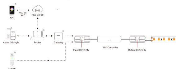
Application Diagram
