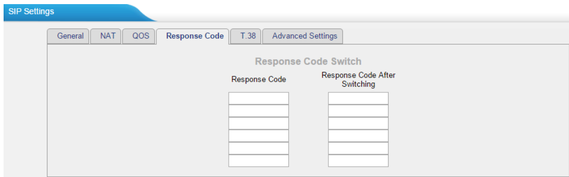
Figure 5-7 Response Code
