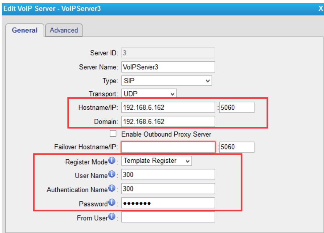
Figure 5-2 Template Register
