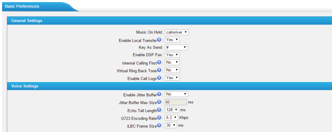
Figure 6-1 Basic Preferences
