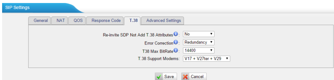
Figure 5-8 T.38 Settings
