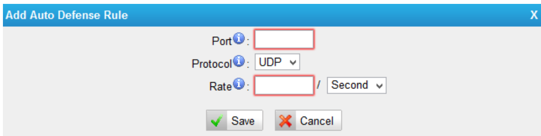
Figure 10-9 Auto Defense
