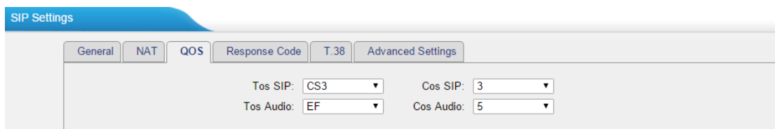
Figure 5-6 Qos
