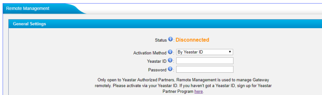
Figure 9-14 Remote Management
