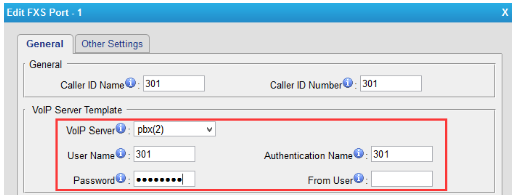
Figure 5-1 Port Register
