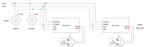
Wiring diagram
